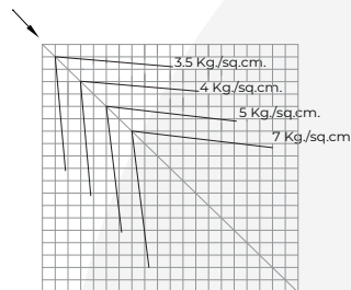
SPRAY AT 45° DOWNWARD
