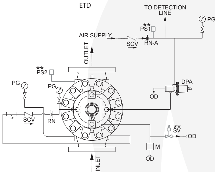
SCHEMATIC2
