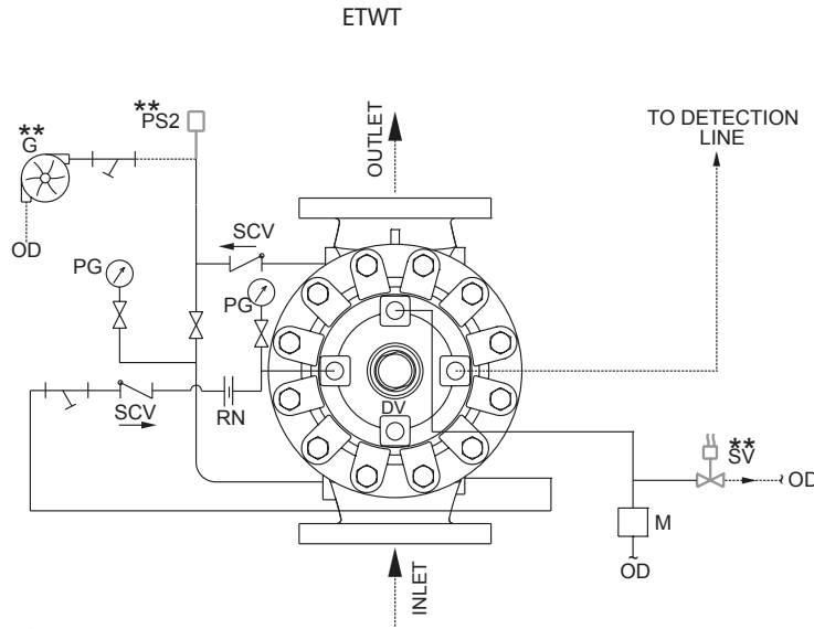
SCHEMATIC 3
