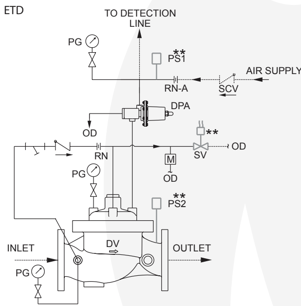
SCHEMATIC 10
