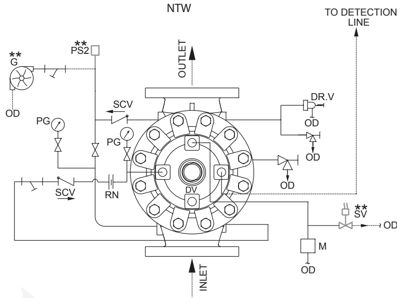
SCHEMATIC 7
