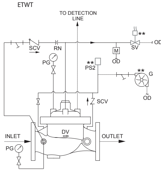
SCHEMATIC 11
