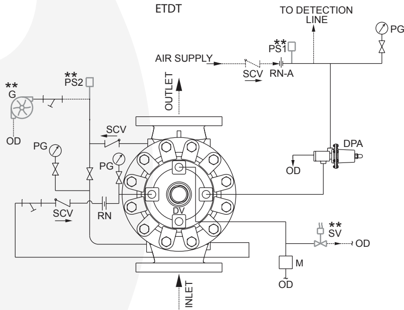
SCHEMATIC 4
